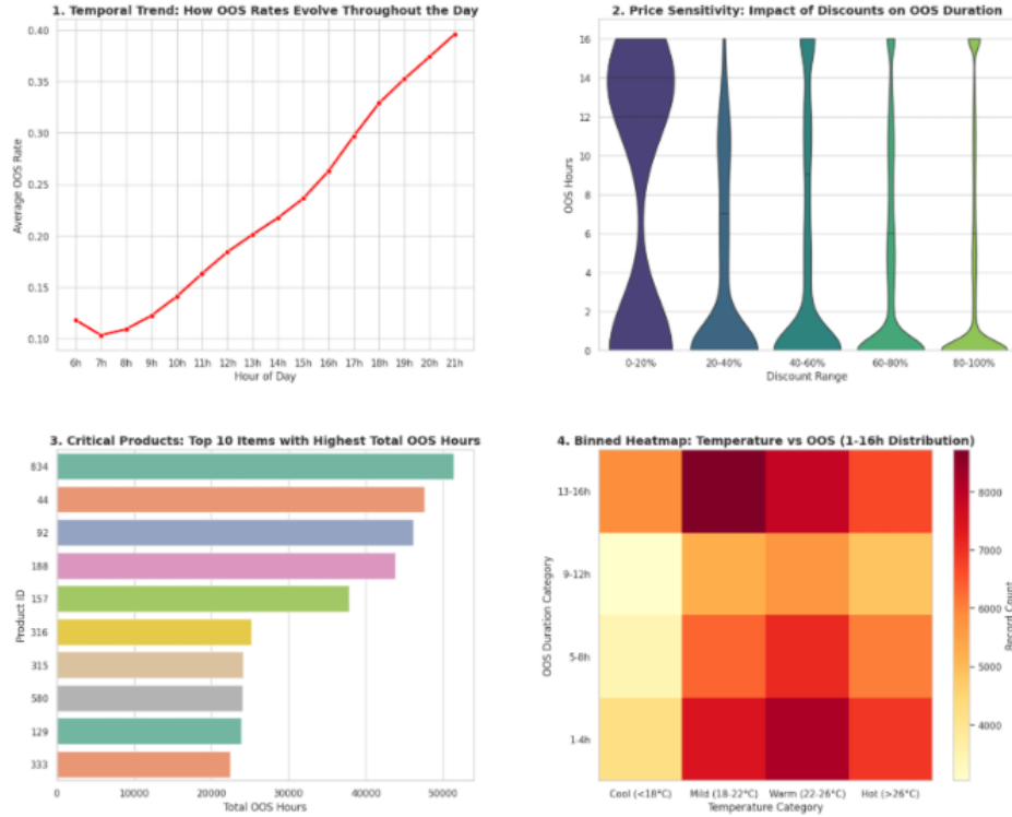
Fig. 2. Bivariate analysis illustrating the impact of time, promotional events, specific SKUs, and temperature on Out-of-Stock durations.
