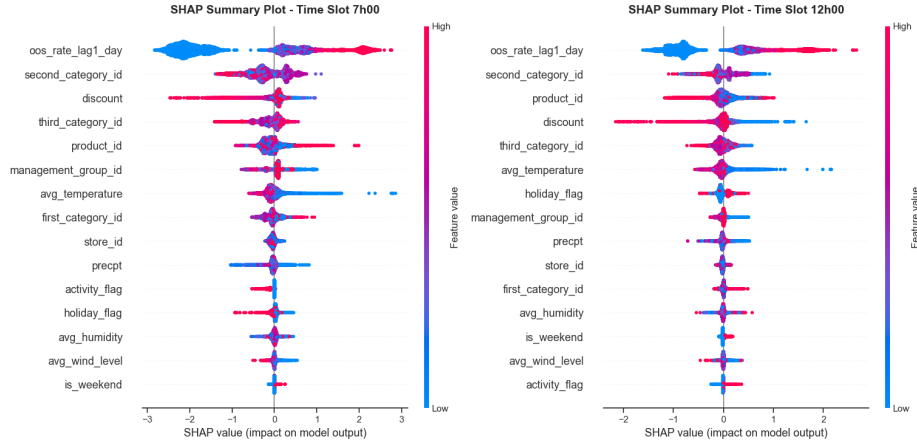
Fig. 4. SHAP impact on OOS probability at 07:00. Fig. 5. SHAP impact on OOS probability at 12:00.
